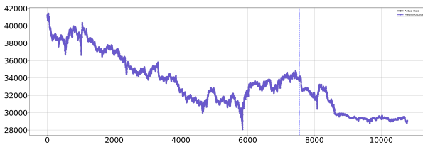
Fig. 6. One-Step Prediction Plot for Neural ODE from 0 to 10783 days
