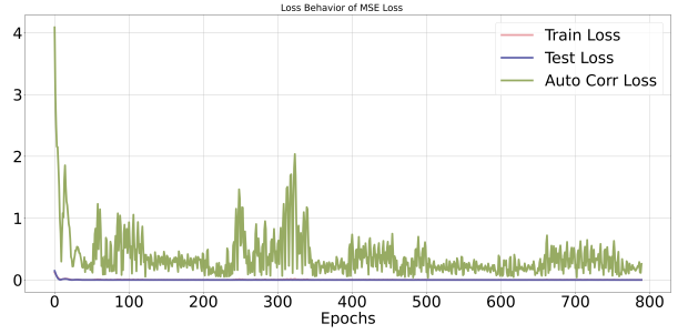
Fig. 10. Loss Plot for N-CATS
