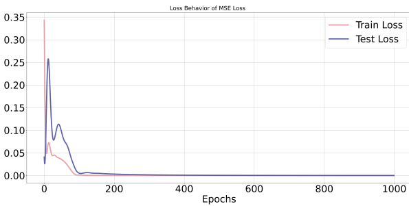
Fig. 8. Loss Plot for LSTM
