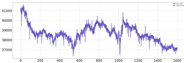
Fig. 7. One-Step Prediction Plot for N-CATS from 0 to 1600 days
