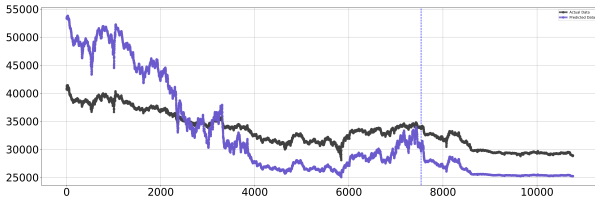
Fig. 5. One-Step Prediction Plot for LSTM from 0 to 10783 days
