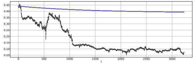
Fig. 11. Multi-Step Prediction for Neural ODE on Unseen Data
